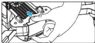
5.1 Buckle the battery lock of the aircraft.
